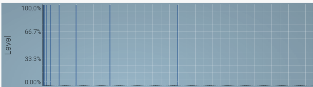
Magnitudes graph
